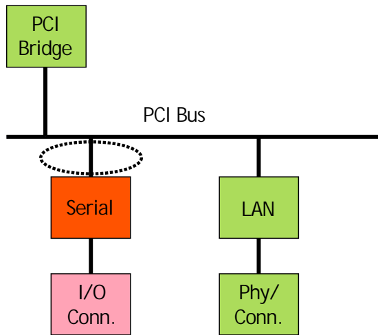
Fig. 6a – Partial PCI Bus failure.
