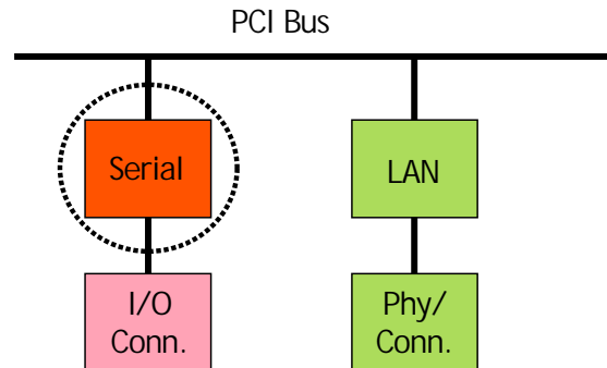
Fig. 6c – Faulty Serial Controller.
