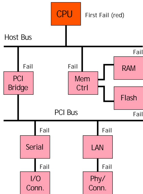
Fig. 2 – Processor Area failure.
