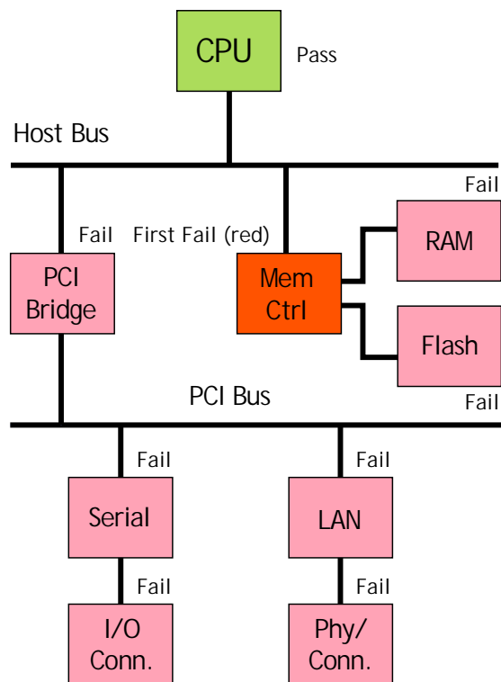
Fig. 3 – Processor Area failure.
