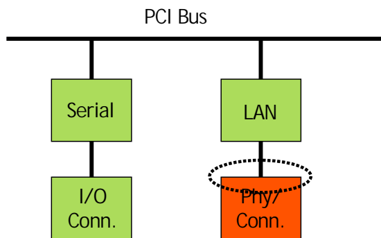
Fig. 7c – Faulty LAN Port Connector.
