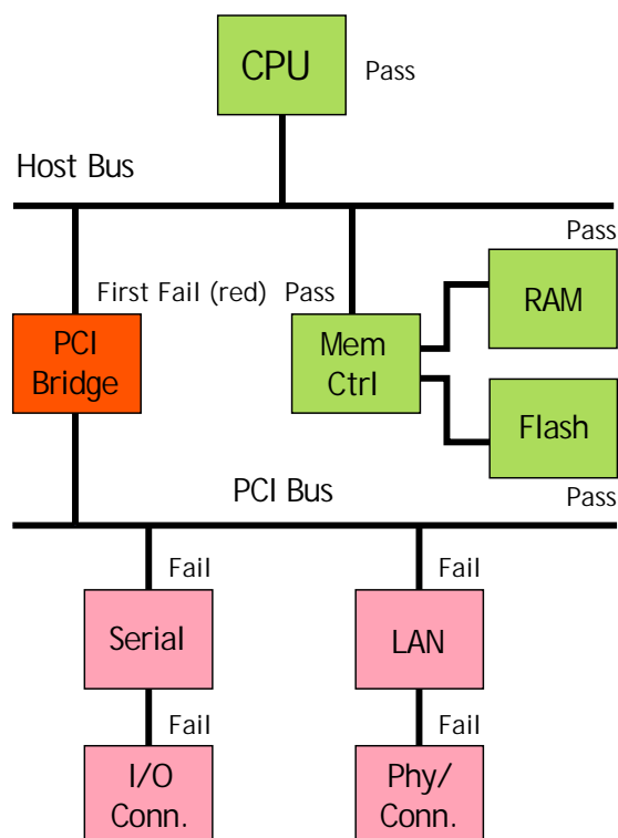
Fig. 4 – Bridge failure.
