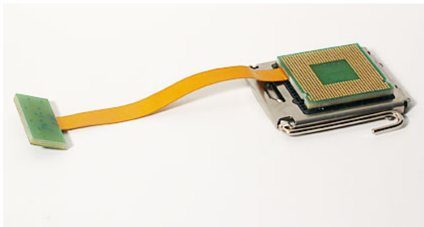
Figure 2.03 Bottom view of the LGA interposer, showing the CPU-shaped PCB that locates into the on-board LGA socket
